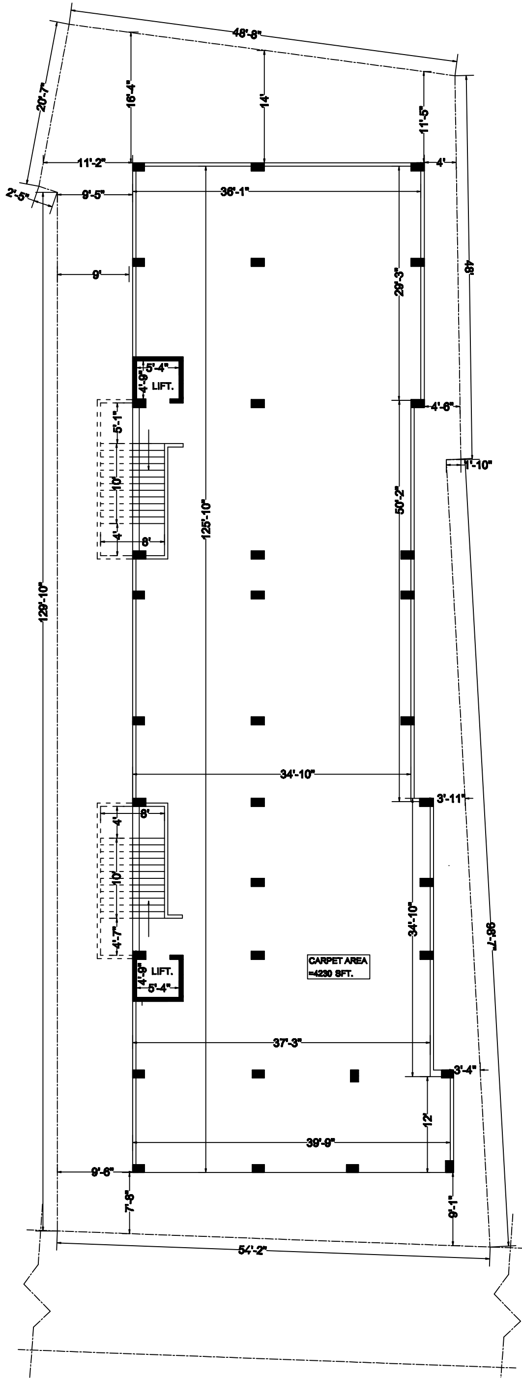
GR. FLOOR PLAN SCALE- 1"=8'-0" TOTAL AREA = 4630 SFT.
